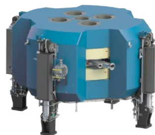
Best Model B35ADP Alpha/Deuteron/Proton Cyclotron
